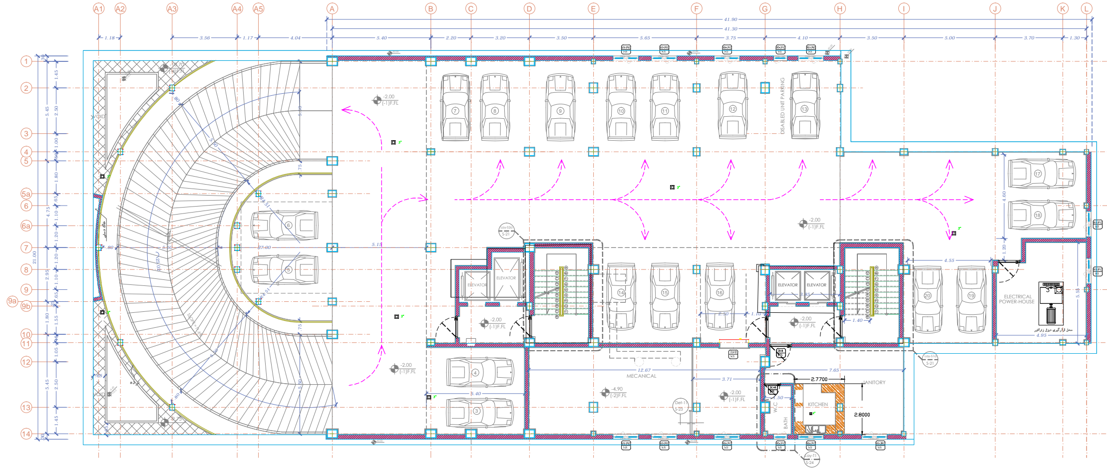
-1st. BASEMENT PLAN
